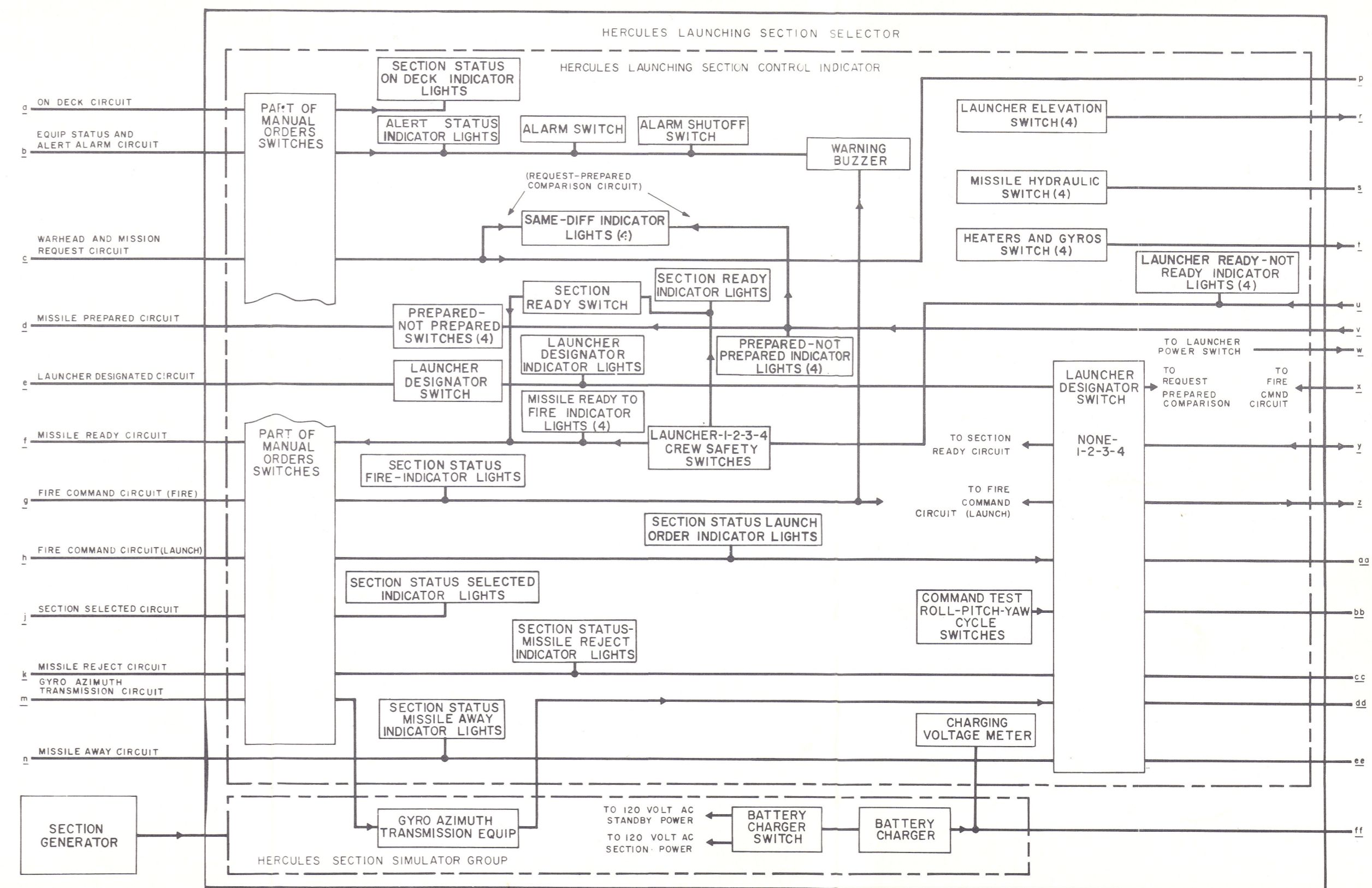
Figure 32 (Sheet 1 of 2). Guided missile launching set—block diagram.
